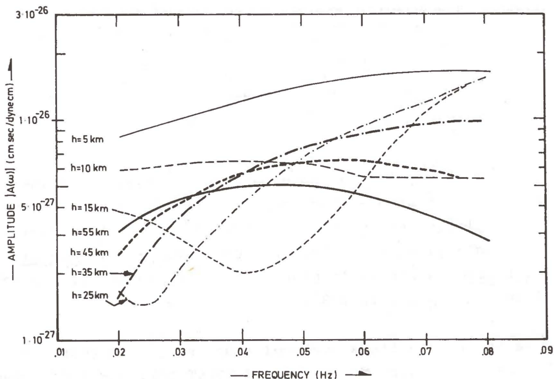
Fig. 4 Dependence of amplitude spectrum of Rayleigh waves on focal depth. The model is the Mohn's ridge earthquake recorded at Kongsberg (KON).
