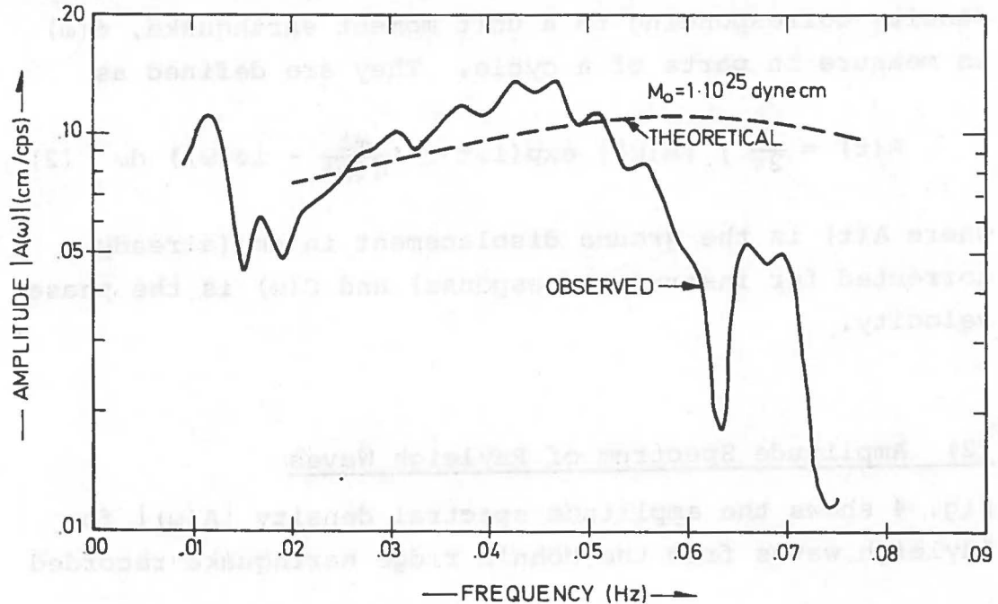
Fig. 3 Comparison of observed and theoretical Rayleigh wave spectra. The Rayleigh waves were recorded at KON for the Mohn's ridge earthquake of 31 May 1971. The fault plane solution of Conant (1973) was used in the theoretical calculations, assuming a focal depth of 8 km. Fault plane strike is N42°E with dip angle 54°, auxiliary plane strike is N52°E with dip angle 64°.
