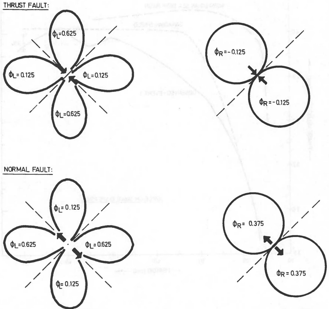
Fig. 7 Source phases for Love and Rayleigh waves for simple fault geometrics, i.e., dip-slip on an inclined fault.
