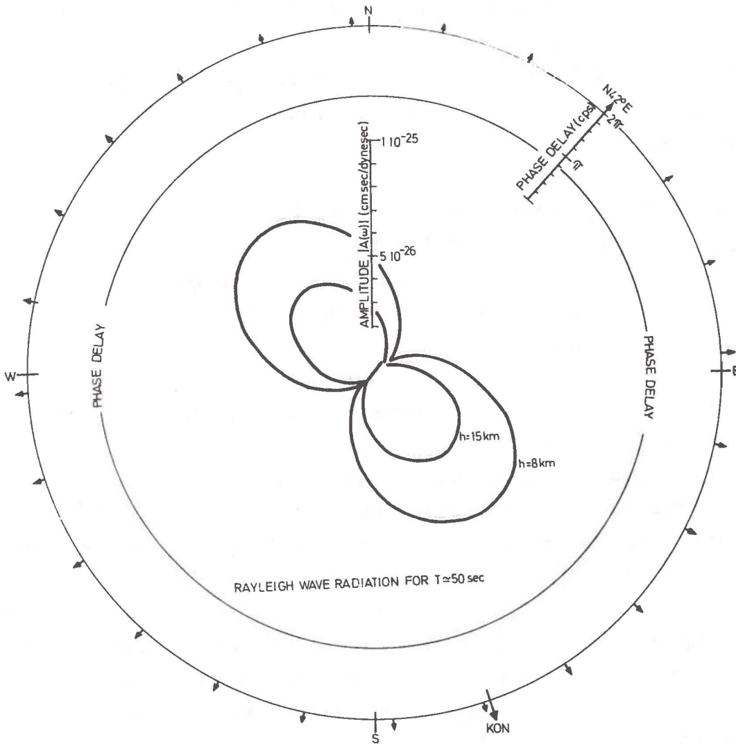
Fig. 5 Rayleigh wave radiation from the Mohn's ridge earthquake. For details on focal parameters see the caption of Fig. 3.
