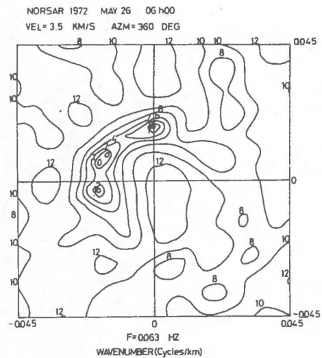
Fig. 4 Wave-number spectra for the 1st and 2nd peak frequencies for four different storms.
