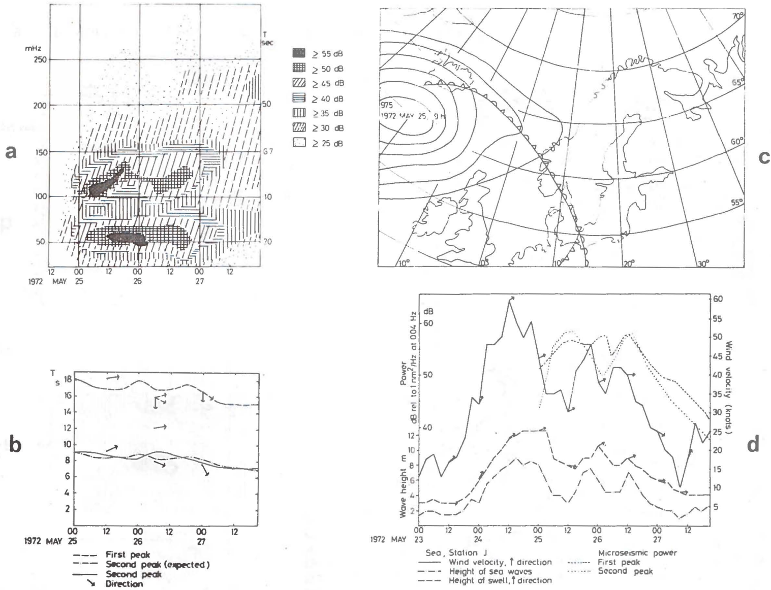
Fig. 10 Pictorial synopsis of Storm 6. See caption for Fig. 5.
