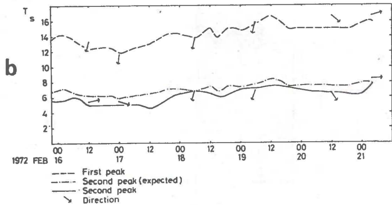
Fig. 6 Pictorial synopsis of Storm 2. See caption for Fig. 5.
