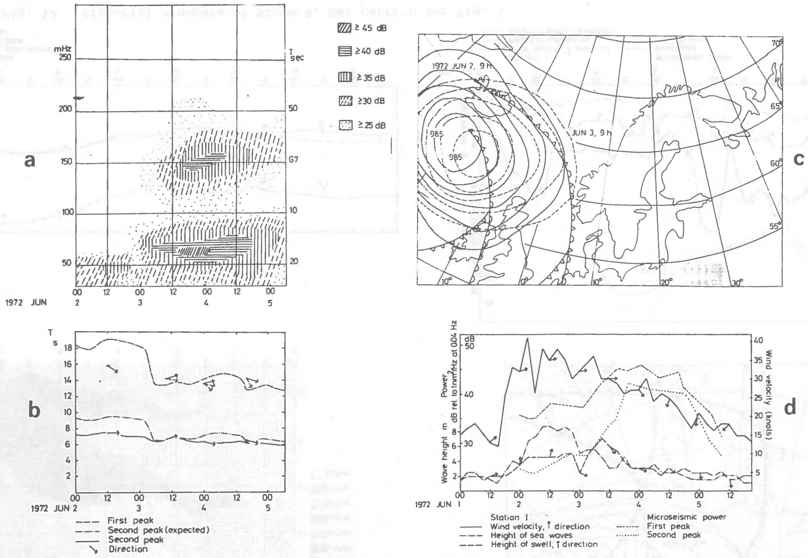
Fig. 11 Pictorial synopsis of Storm 7. See caption for Fig. 5.
