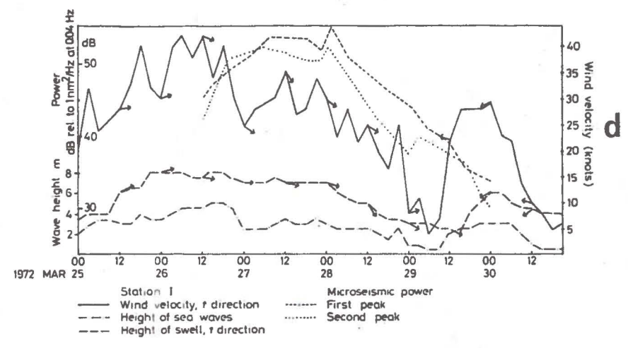
Fig. 8 Pictorial synopsis of Storm 4. See caption for Fig. 5.
