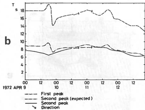
Fig. 9 Pictorial synopsis of Storm 5. See caption for Fig. 5.
