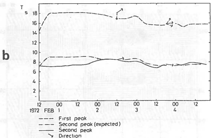
Fig. 5 Pictorial synopsis of storm 1. a) Sonogram illustrating power spectral variations during storm progression. b) Variation with storm progression of the periods of the 1st and 2nd spectral peaks and also the half period of the 1st peak (see legend). Arrows indicate the direction (relative to N) of coherent microseismic waves. c) Weather map representative of this storm. d) Comparison of data from weather ship and power variations of the 1st and 2nd microseismic peak (see legend).
