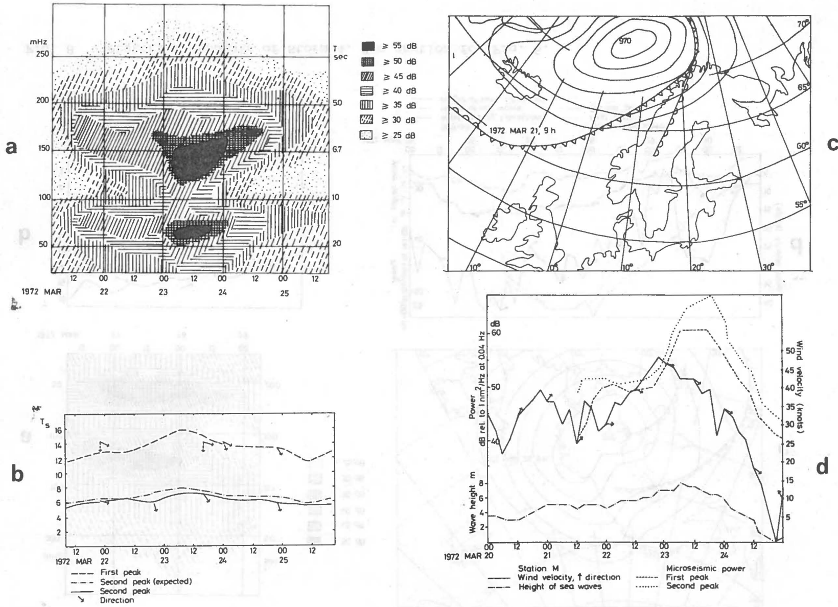
Fig. 7 Pictorial synopsis of Storm 3. See caption for Fig. 5.
