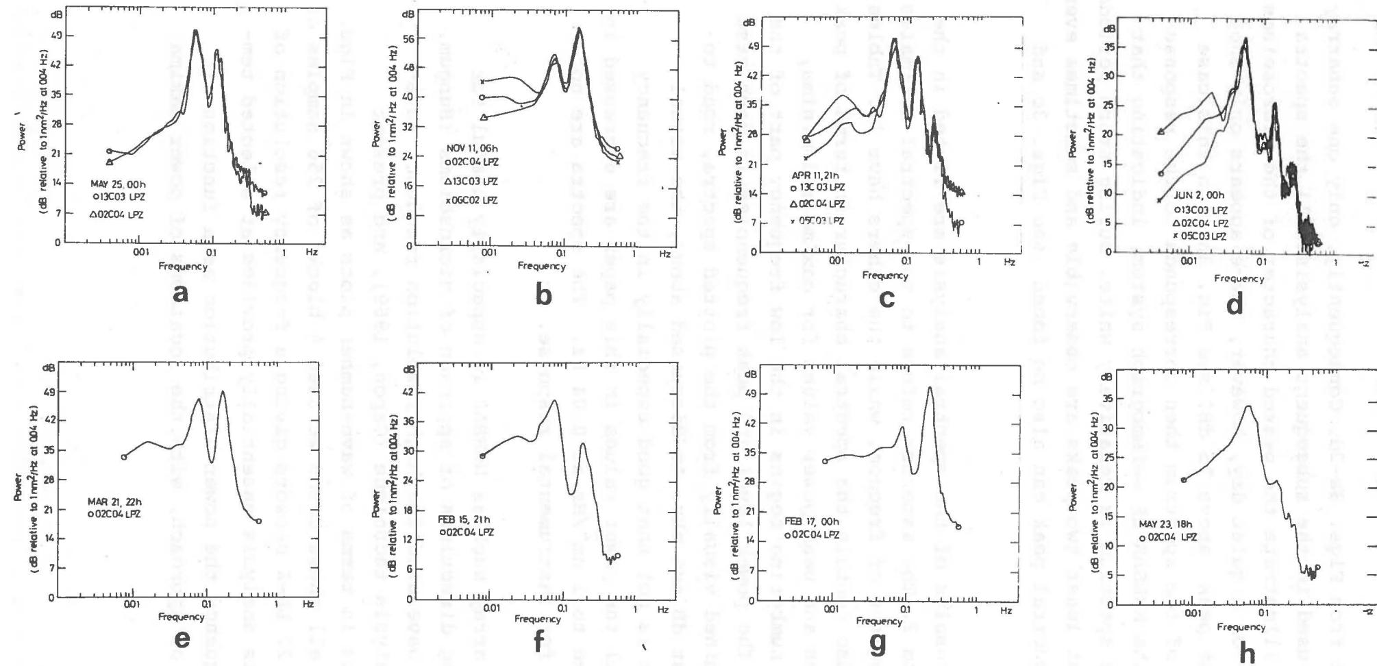
Fig. 3 Typical power spectra computed from NORSAR LP-Z recordings during stormy periods (a-g) and on a quiet day (h). In frames a-d spectra obtained from 2 or 3 different sites within NORSAR are superimposed for comparison. The spectral estimates in frames a, c, d, g, h have 16 degrees of freedom and in frames b, e and f 40 degrees of freedom.
