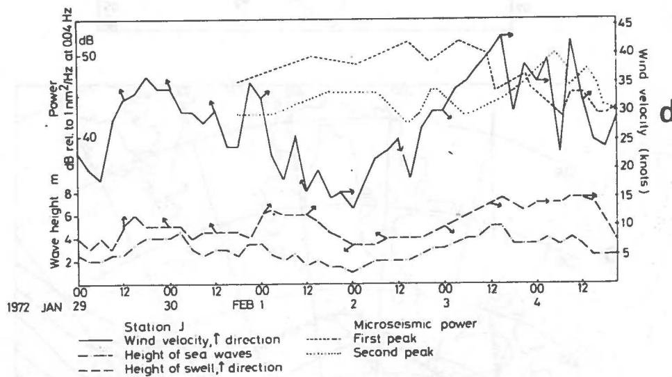
Fig. 5 Pictorial synopsis of storm 1. a) Sonogram illustrating power spectral variations during storm progression. b) Variation with storm progression of the periods of the 1st and 2nd spectral peaks and also the half period of the 1st peak (see legend). Arrows indicate the direction (relative to N) of coherent microseismic waves. c) Weather map representative of this storm. d) Comparison of data from weather ship and power variations of the 1st and 2nd microseismic peak (see legend).
