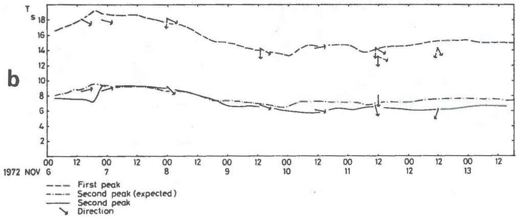
Fig. 12 Pictorial synopsis of Storm 8. See caption for Fig. 5.
