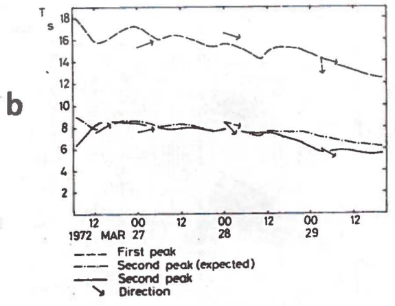
Fig. 8 Pictorial synopsis of Storm 4. See caption for Fig. 5.
