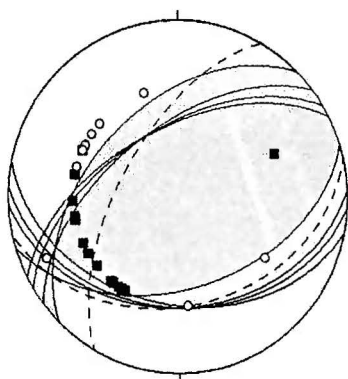
Fig. 6.6.6. This figure shows the initial focal mechanism solution for the Revda event derived from 28 first motion readings from Fennoscandia (filled symbols are compressions, open symbols dilations), with several possible solutions (courtesy of Erik Hicks), used as starting solution for the waveform modelling. The shaded solution is the final one following a systematic search over mechanism parameter space. The parameters for the final solution are shown to right.
