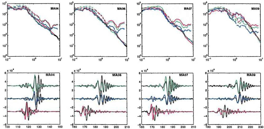
Fig. 6.6.7. Observations and synthetics for model 2 and a source depth of 5 km computed with the f-k method. Top: signal (solid) and modelled (dashed) amplitude spectra (in [nm s]) for the frequency range between 0.1 and 10 Hz, Green, blue and read are the vertical, radial and transverse component, respectively. Bottom: Observed displacement (color coded as above) and modelled displacement (black)
