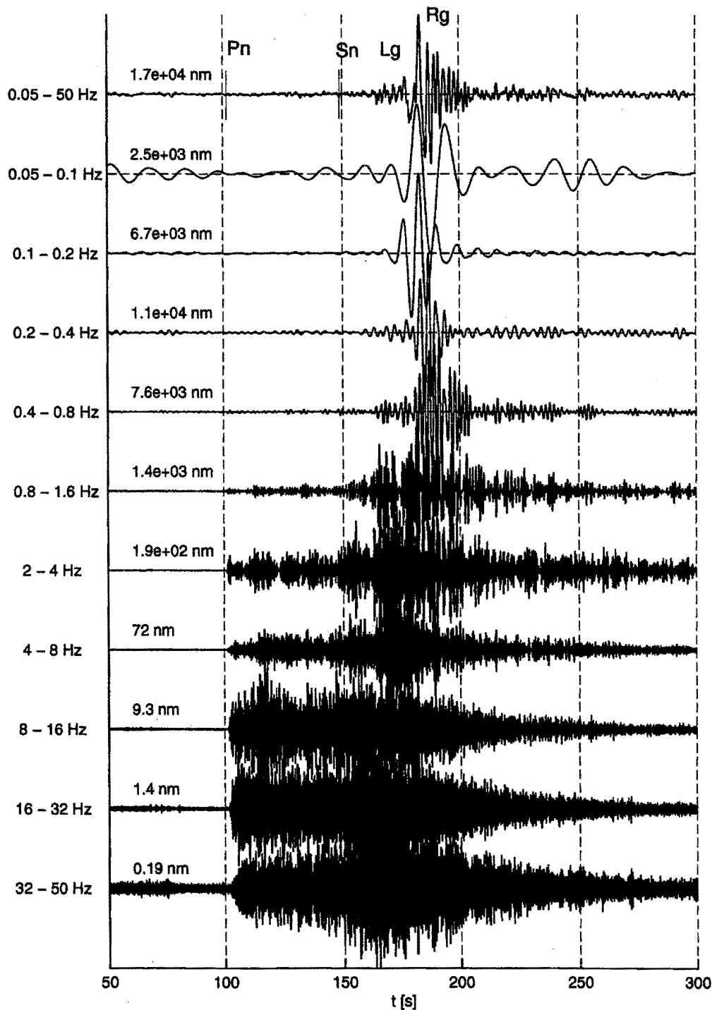
Fig. 6.6.3. Displacements recorded at station MA06 for different frequency bands. See the main text for more details and discussion.
