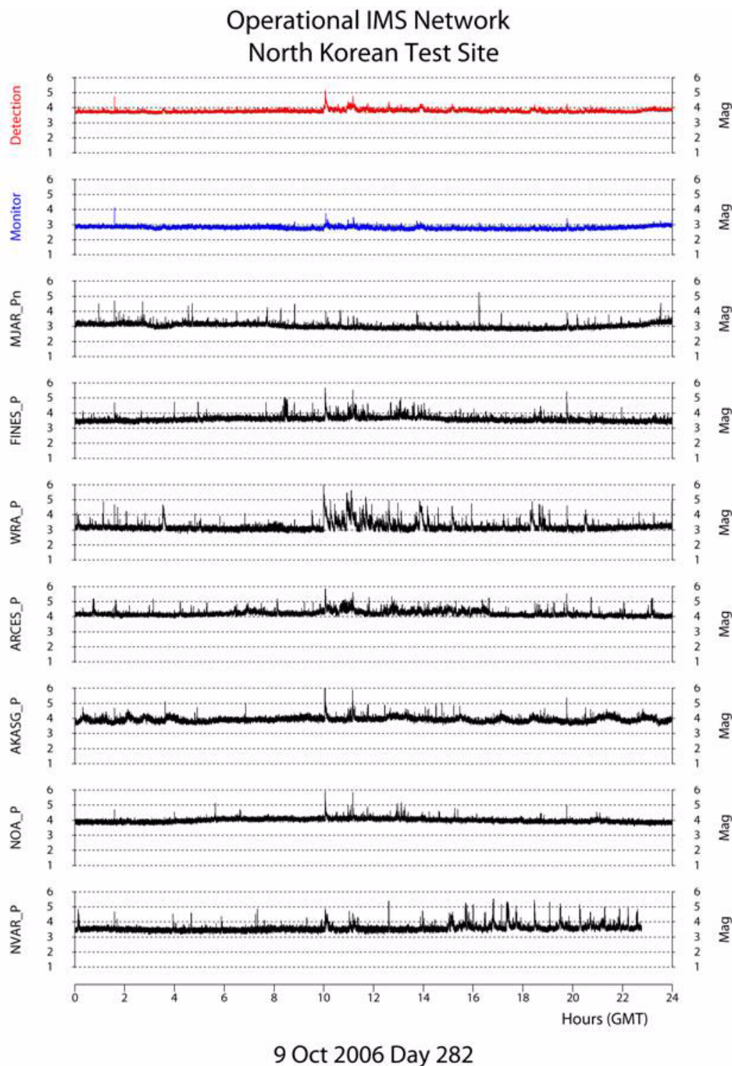
Fig. 6.1.5. Threshold monitoring results for the day of the nuclear test (9 October 2006). In this figure we have used only those of our selected stations that were operational at the IDC during that day. Detection thresholds (red) are close to magnitude 4.0 or slightly below, except for occasional increases during the nuclear test (at 01.35) and during some interfering events later in the day. The monitoring thresholds (blue) average about magnitude 3.0. The individual station P-thresholds (black) are also shown.
